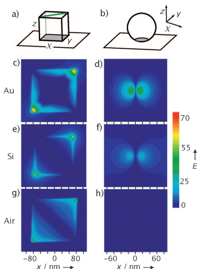
Figure 4. Simulated E-field enhancements for a Ag nanocube or nanosphere. a,b) Coordination systems for calculating the E-field enhancement distribution of a nanocube and nanosphere, respectively, positioned 2 nm above a substrate. The gray region represents the plane plotted in the simulations and is 1 nm above the underlying substrate. For nanocubes, the polarization was along the green line. The E-field enhancement distributions calculated using the DDA method for: nanocubes c) on Au, e) on Si, and g) in air; as well as for nanospheres d) on Au, f) on Si, and h) in air.
